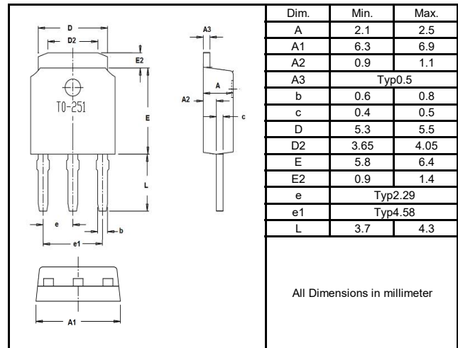
T0-251
