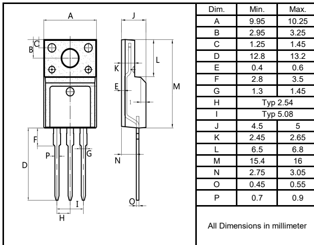
T0-220F
