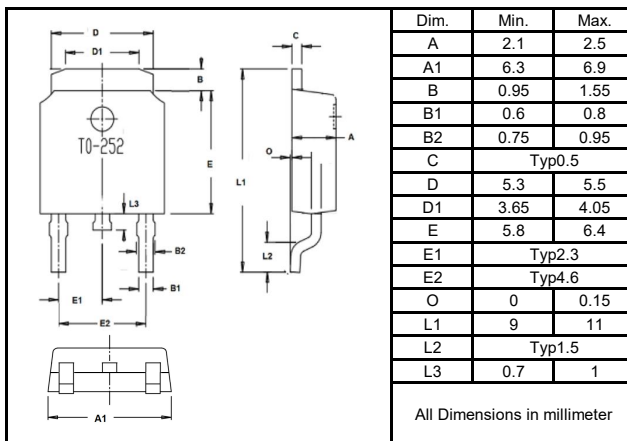
T0-252
